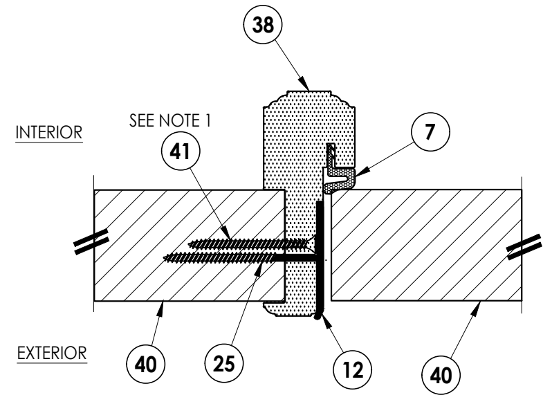
4 5 HORIZONTAL CROSS SECTION Outswing shown (Inswing similar)
